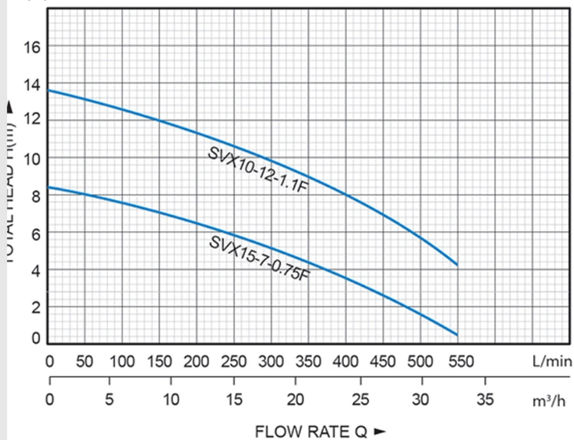
H(m) Performance chart at n=2860 r/min
