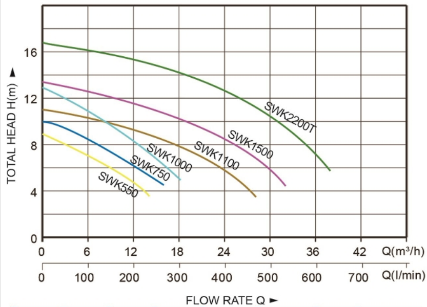
H(m) Performance chart at n=2860 r/min
