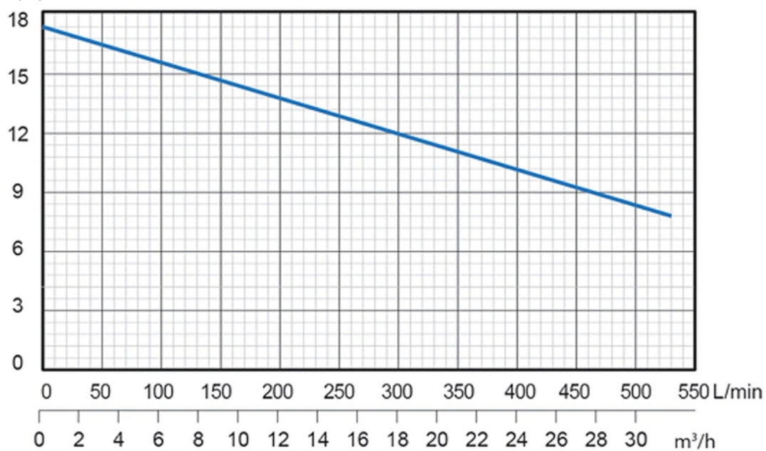
H(m) Performance chart at n=2860 r/min
