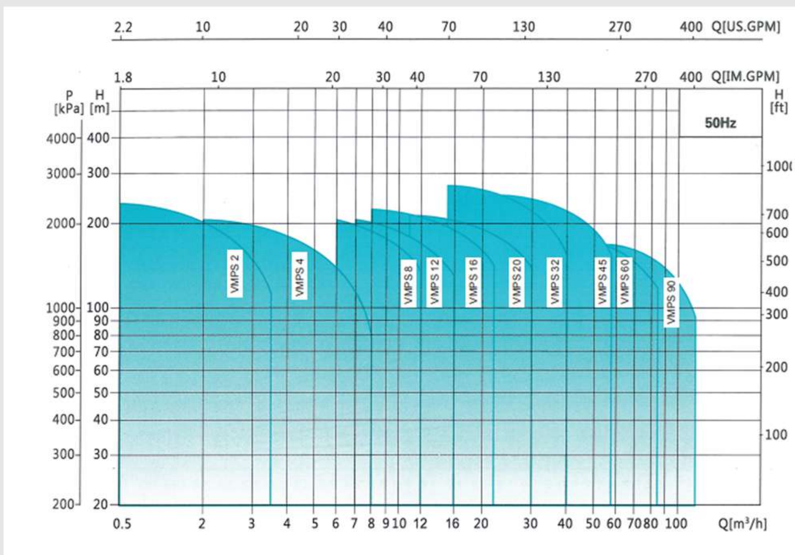
Three phase Motor at 50 Hz, 2 poles
